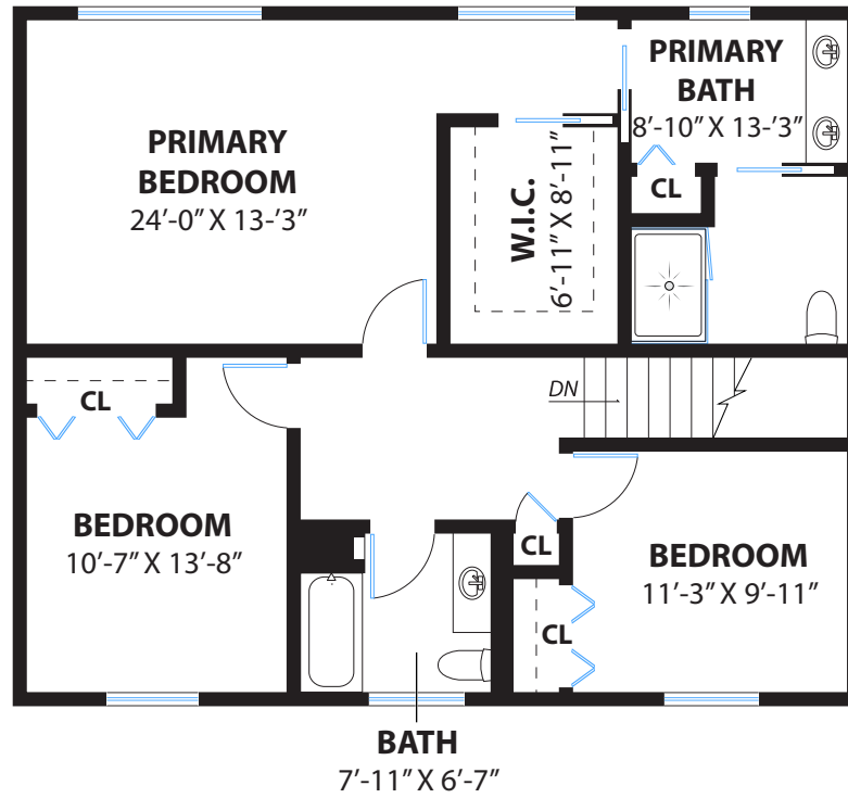
UPPER FLOOR
